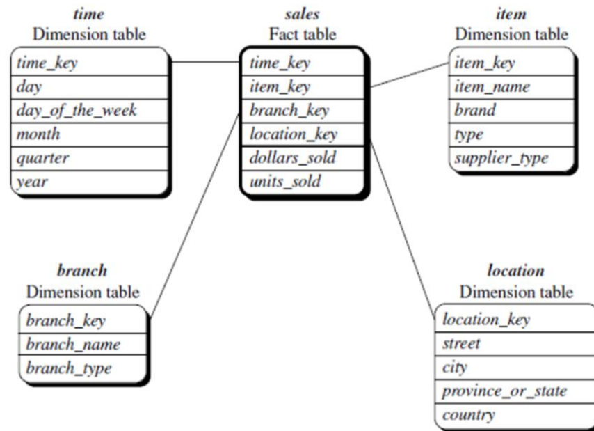
figure : Star schema of sales data warehouse.
