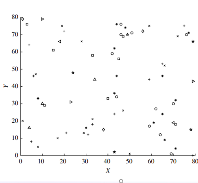
Figure : Visualization of a 2-D data set using a scatter plot
