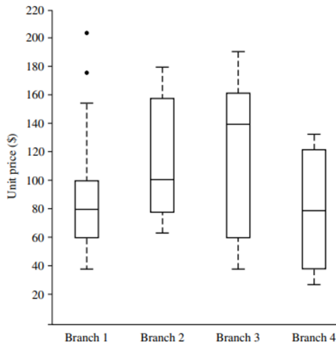
figure: Boxplot for the unit price data for items sold at four branches of AllElectronics during a given time period.
