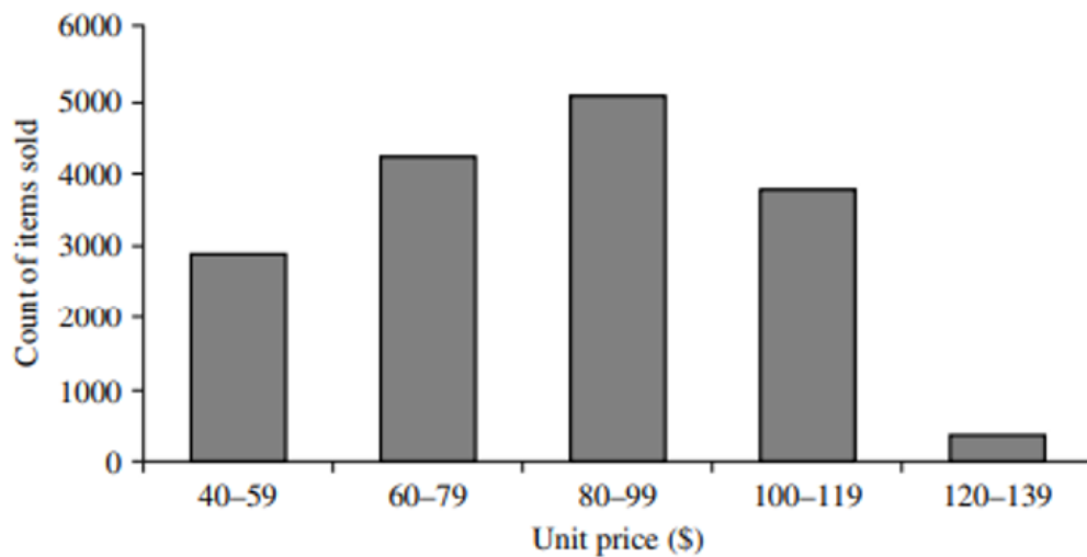
Figure: A histogram for the above Table data set.
