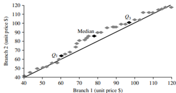
Figure A q-q plot for unit price data from two AlIElectronics branches.
