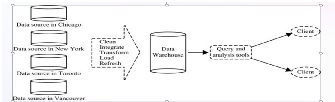
figure: An Architecture of Data Warehouse for All Electronics
