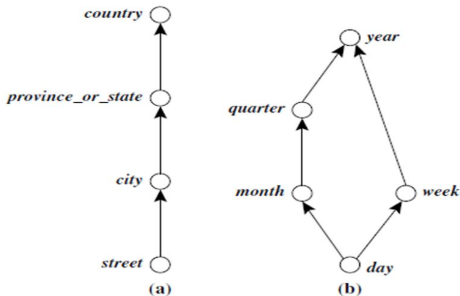
(a) a hierarchy for location and (b) a lattice for time.
