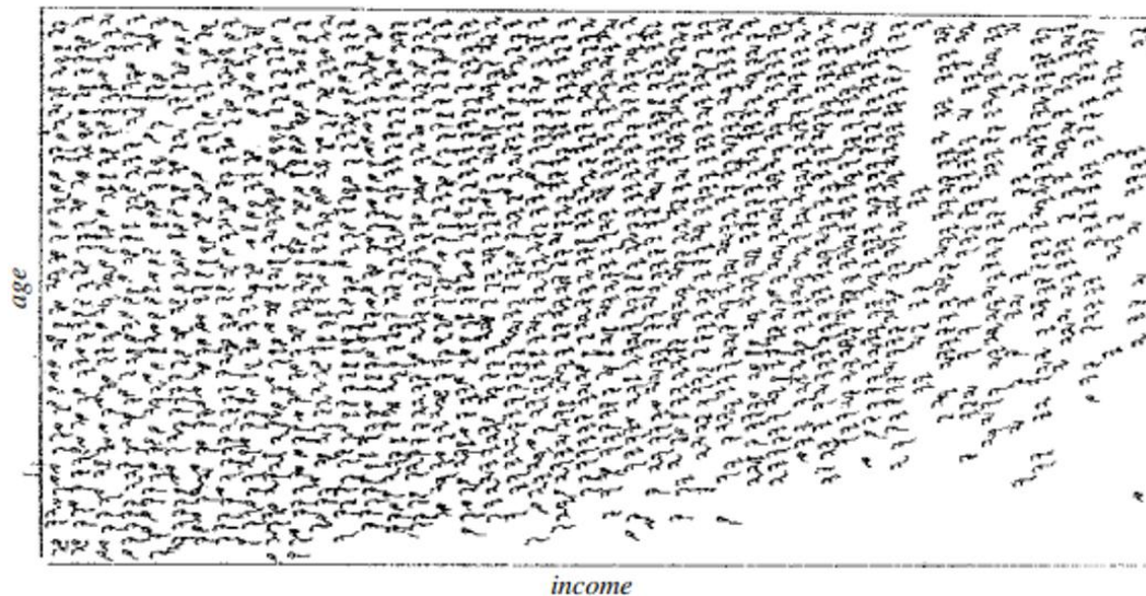
Figure : Census data represented using stick figures
