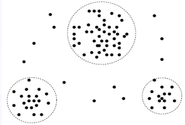
Customer data with respect to customer locations in a city, showing three data clusters.
