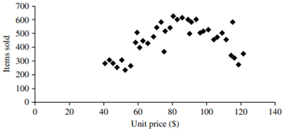
Figure : A scatter plot for the above Table data set.
