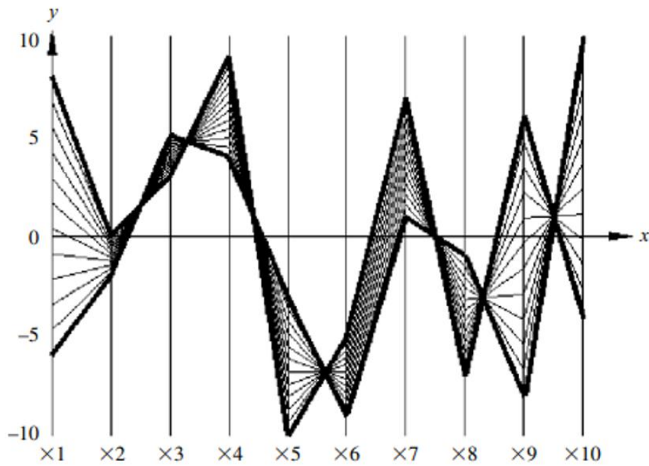
Figure: Here is a visualization that uses parallel coordinates
