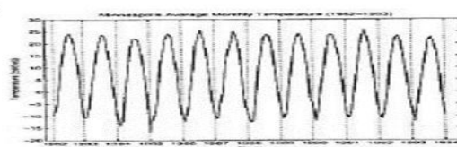
(c) Temperature time series.
