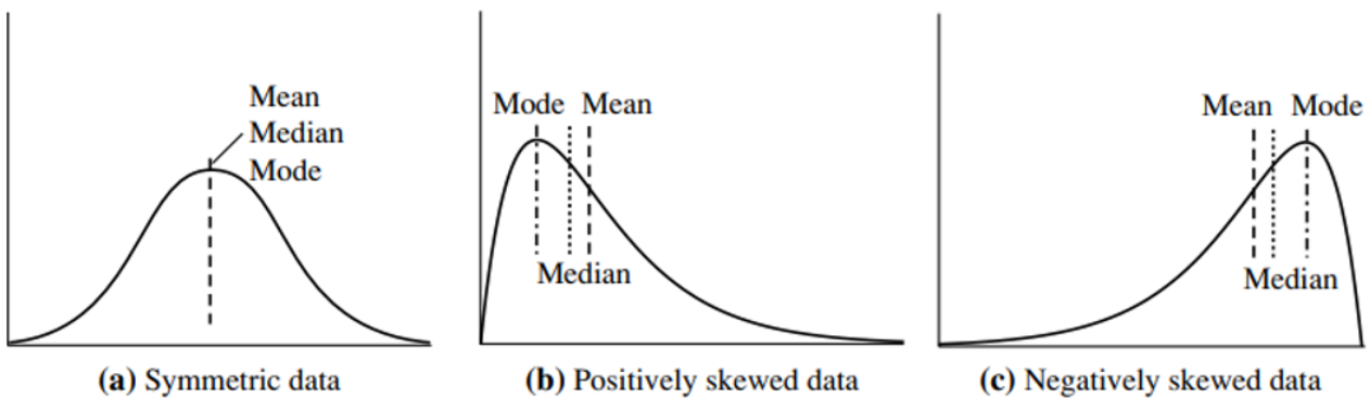
Figure :Mean, median, and mode of symmetric versus positively and negatively skewed data.
