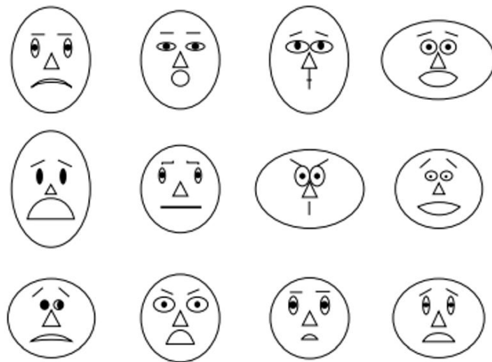
Figure: Chernoff faces. Each face represents an n -dimensional data point ( n \leq 18 ).
