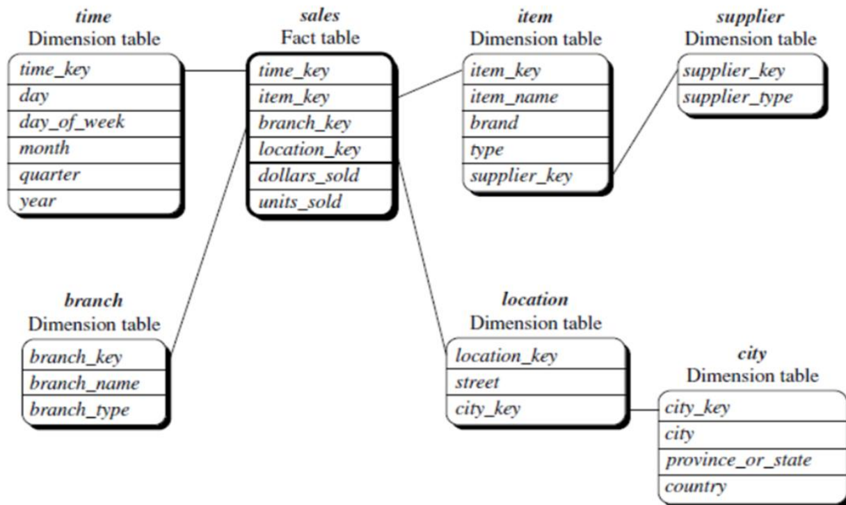
Figure: Snowflake schema of a sales data warehouse.
